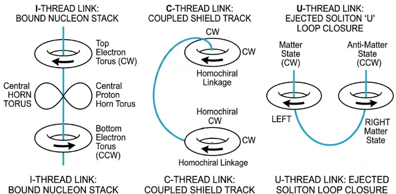
Figure 1: The ICU Topological Pair Genesis Taxonomy: (I) Inter-species Baryon-Lepton coupling forming a bound nucleon stack. (C) Homochiral Intra-species entanglement (Baryon-Baryon or Lepton-Lepton) linked by a subterranean Falaco thread. (U) Heterochiral Matter-Antimatter pair production born from the bifurcation of a sheared U-loop mesocyclone base.
